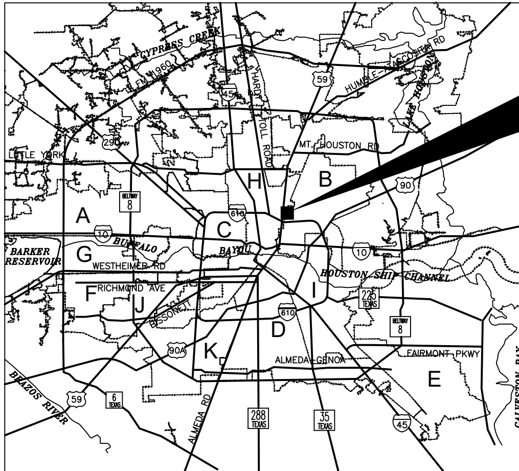
LOCATION MAP
