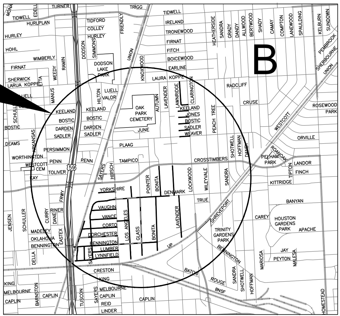
VICINITY MAP
