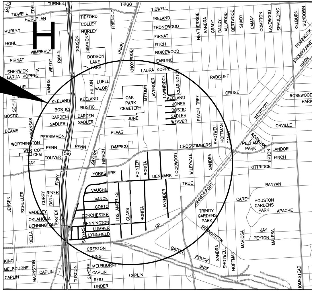
VICINITY MAP
